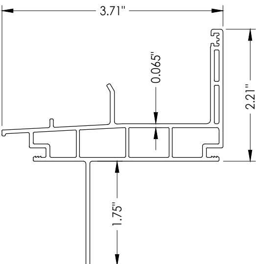
2 SILL
