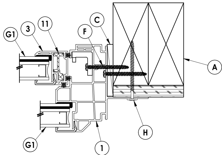
2 HORIZONTAL CROSS SECTION Shown w/ 2X Stud Construction
