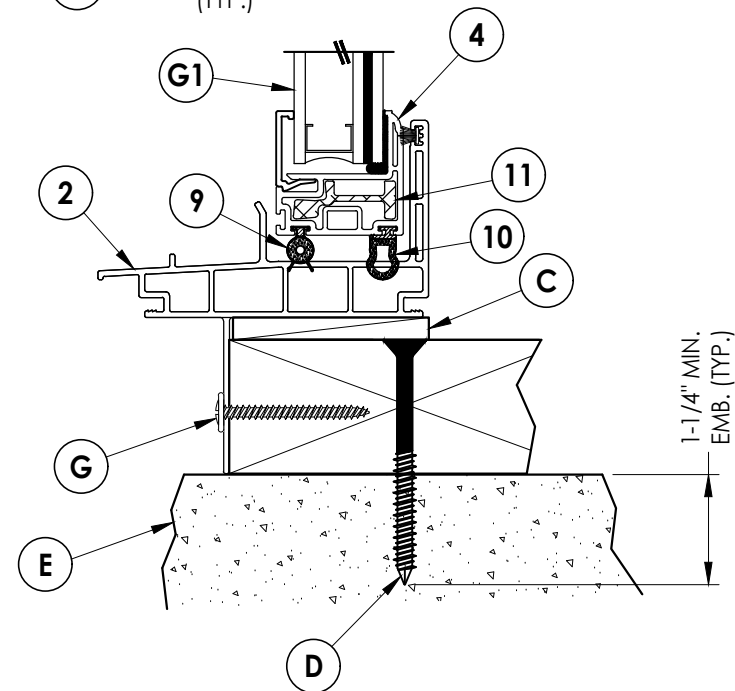
3 HORIZONTAL CROSS SECTION Shown w/ 2X buck
