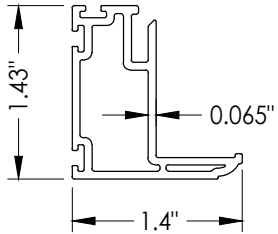
3 SASH STILE
