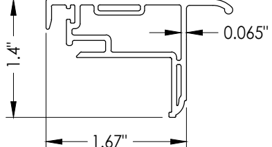
5 LOCK RAIL
