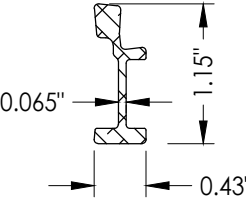
11 SASH REINFORCEMENT
