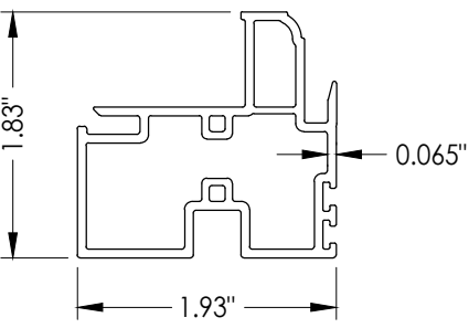
6 KEEPER RAIL
