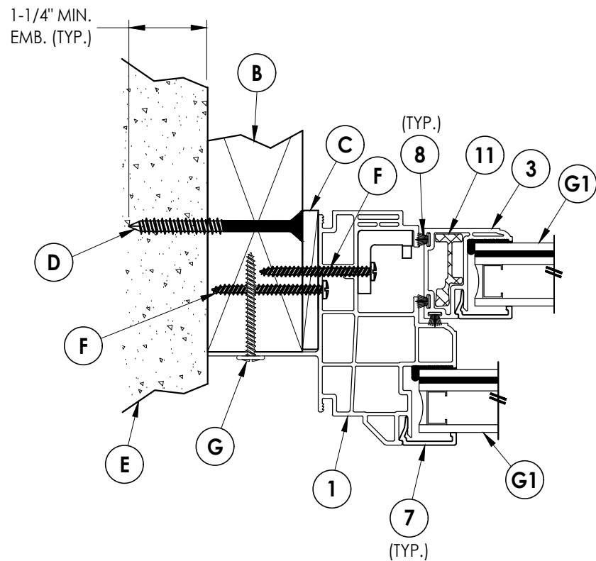
1 HORIZONTAL CROSS SECTION Shown w/ 2X Buck
