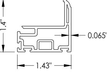
4 SASH BOTTOM RAIL
